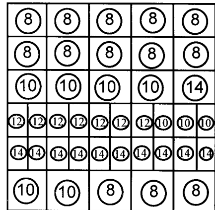
Standard spiral configuration Model 170
